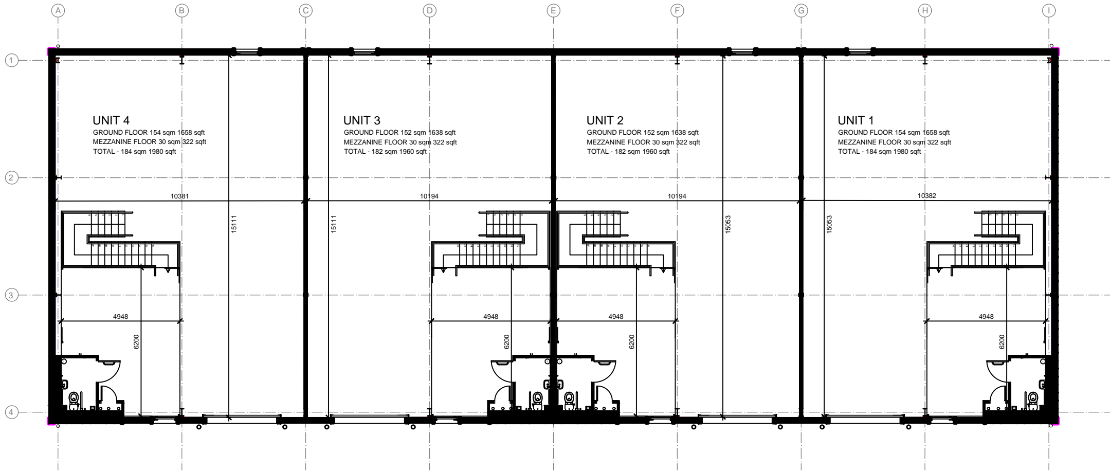
1 GROUND FLOOR PLAN JW/01
